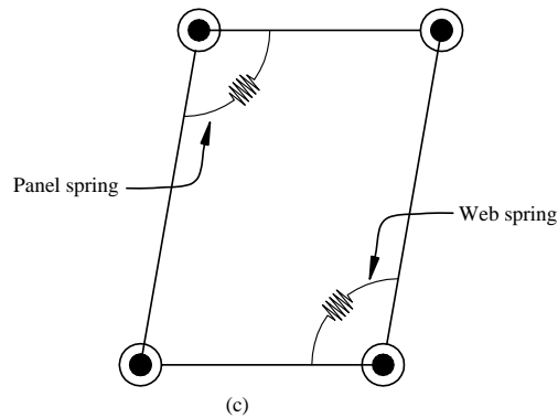
Figure 3.2-14 Transforming shear deformation to rotational deformation in the Krawinkler model.
