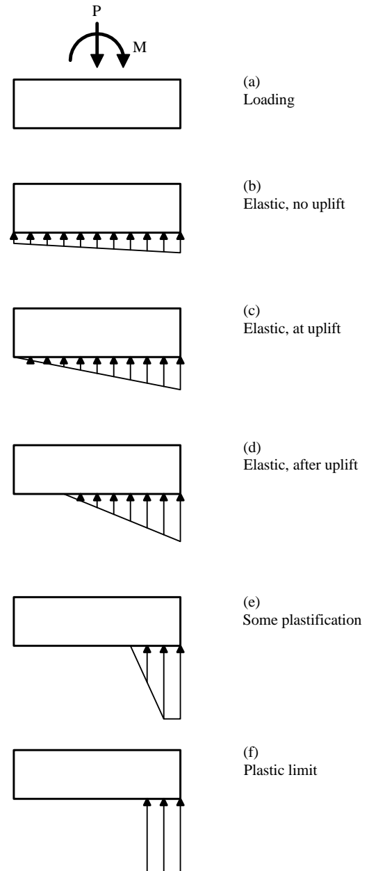
Figure 4.1-3 Soil pressure distributions.
