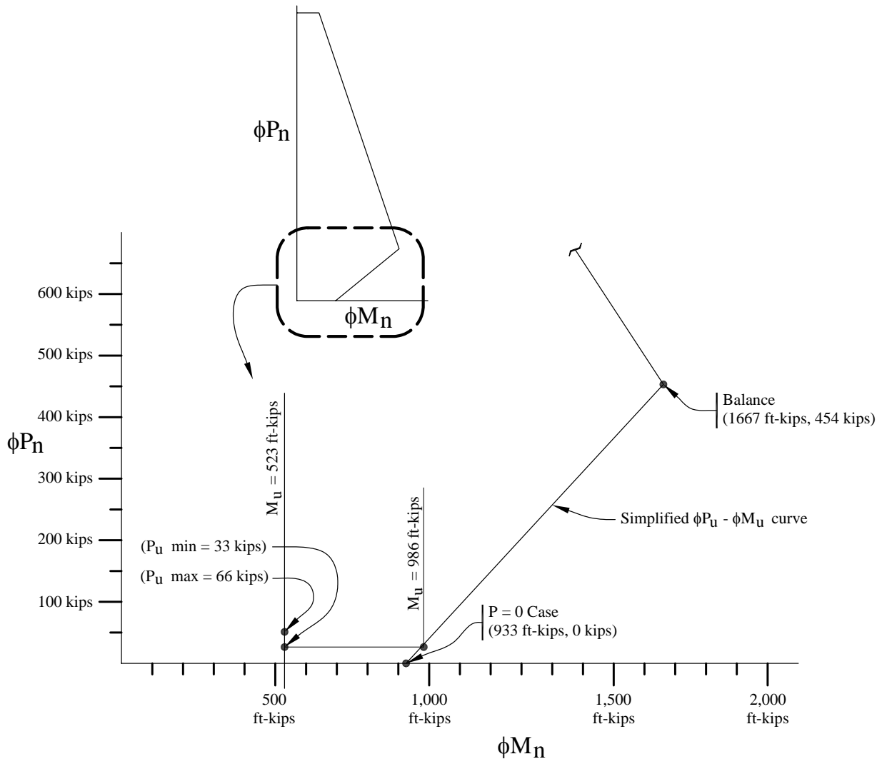
Figure 9.1-21 In-plane \phi P_{11} - \phi M_{11} diagram for pier (1.0 kip = 4.45 kN, 1.0 ft-kip = 1.36 kN-m).
