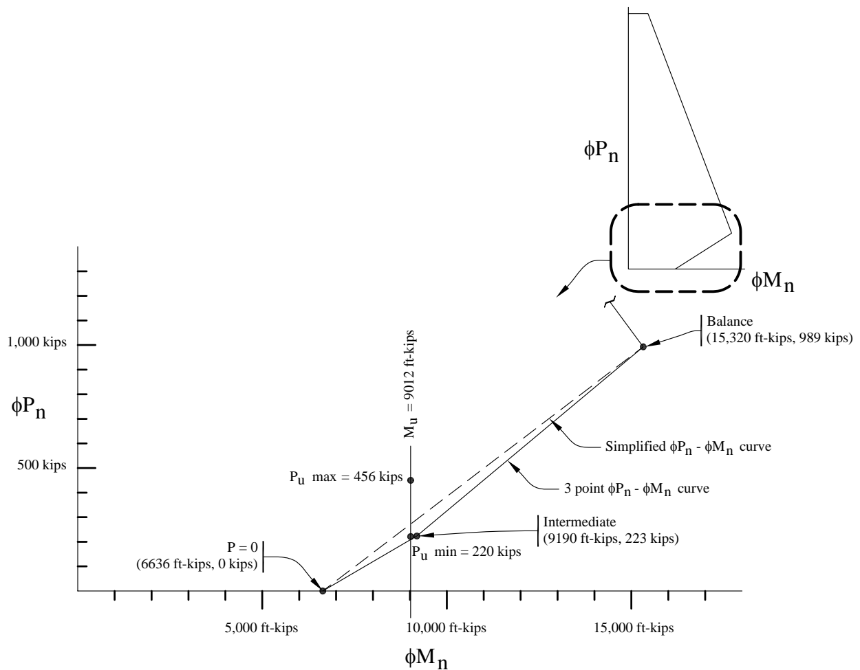
Figure 9.2-14 \phi P_{11} - \phi M_{11} diagram for Los Angeles Wall D (1.0 kip = 4.45 kN, 1.0 kip-ft = 1.36 kN-m).
