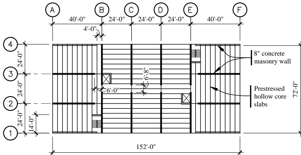
Figure 9.2-1 Typical floor plan (1.0 in = 25.4 mm, 1.0 ft = 0.3048 m).
