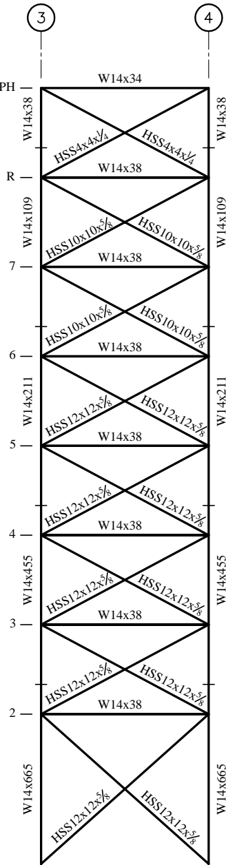
Figure 5.2-17 Braced frame in N-S direction.
