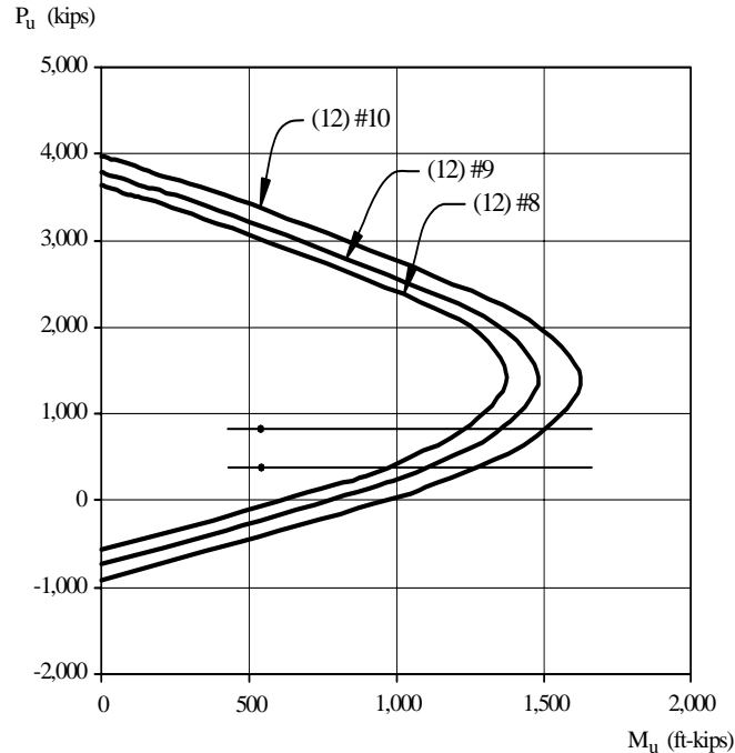
Figure 6-25 Design interaction diagram for column on Gridline A' (1.0 kip = 4.45kN, 1.0 ft-kip = 1.36 kN-m).
