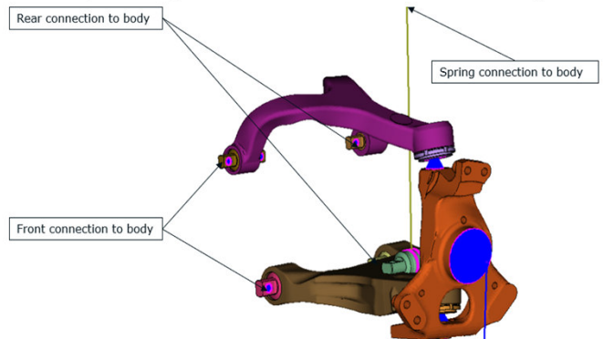
Wheel suspension (front and rear axis with identical suspension)
