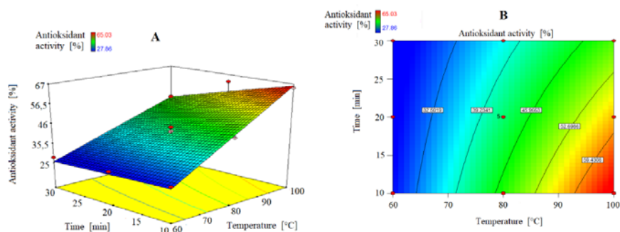
Fig. 2: Three-dimensional response surface (A) AA of horsetail extract with respect to temperature and time and two-dimensional contour diagram (B)
