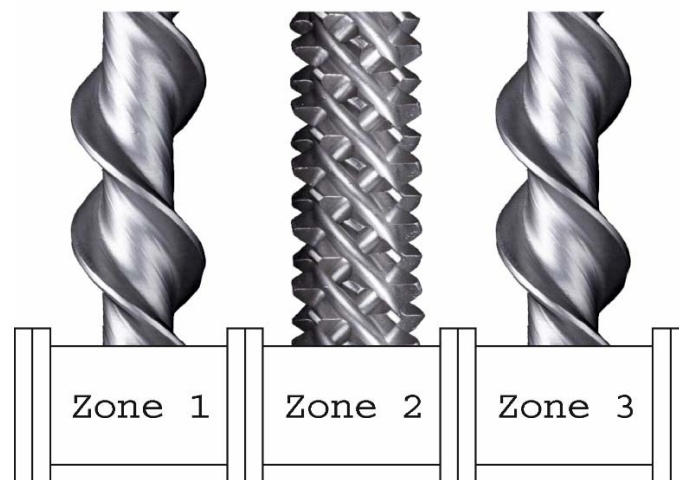
Fig. 2.: Planet spindle profile in the following zones [4]
